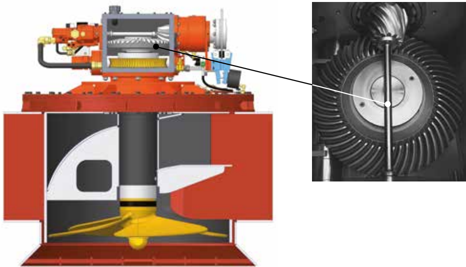
Veth Propulsion uses spiral-cut bevel gears. This type of gear ensures smooth gearing with a lower noise level. The shaft that drives the hydraulic pump is directly connected to the pinion gear; it is one example of the well thought-out design of a Veth Jet. A simple, robust and durable solution for driving the pump.
